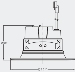
4" Recessed Downlight
