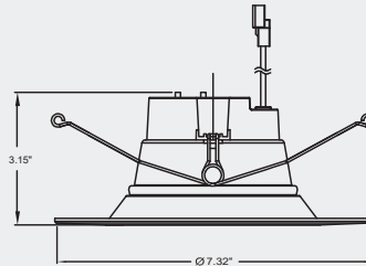
6" Recessed Downlight
