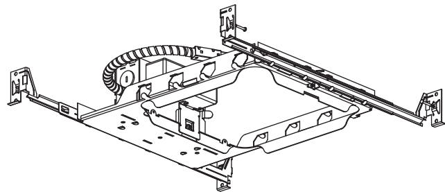
LS-8INCH-SQ-0-10V (0-10V Dimming)
