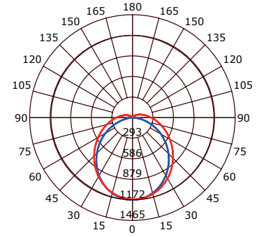
PHOTOMETRIC LS26-N-8FT-3CCT LS26-N-8FT-E-3CCT
