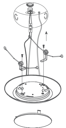
5" & 6" Housing
